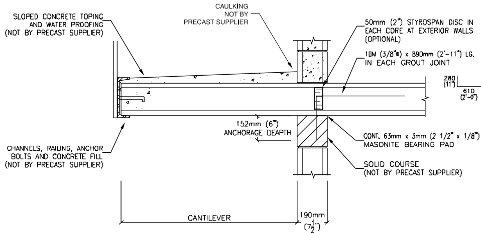
Cantilevered Balcony - Tie Down N.T.S.
