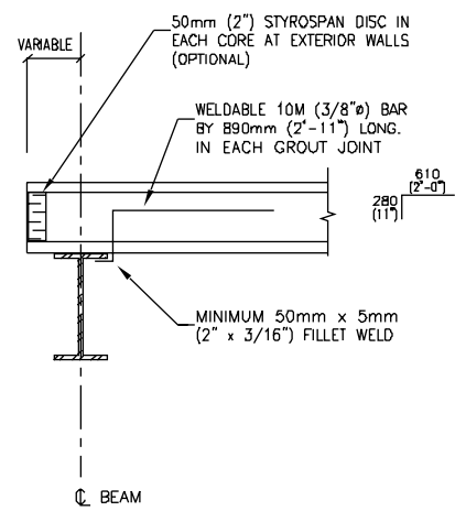
End Bearing On Steel - (63mm or 2fi" min) - Tie Down N.T.S.
